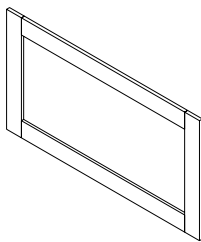
Framed Mirror, Stained Spruce BA058S 80x60x3 cm BA051S 80x80x3 cm BA056S 100x80x3 cm BA061S 130x70x3 cm
