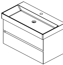
17085 KARE Ceramic Basin 85x45 cm GU083L GODIVA Cast Marble Basin 83x44 cm Vanity Base, 2x Drawer 82x51,5x43 cm FID1285B White Matt FID1285D Oak
