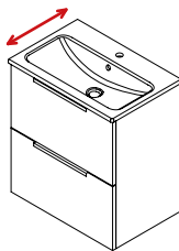
44060 PRACTICO Ceramic Basin 60x40 cm Vanity Base, 2x Drawer 58x54x39 cm CR592-3030 White Glossy CR592-XXXX
