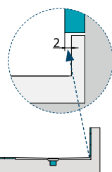
73181 Shower Tray Waste Ø 90 mm, White
