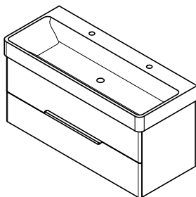
9024211 SAND Ceramic Basin 2 Tap Holes 120x50 cm Vanity Base, 2x Drawer 117x51x48,5 cm MD120 White Matt/White Matt MD121 White Matt/Oak Graphite MD122 White Matt/Oak Natural
