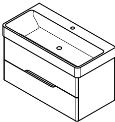
9023111 SAND Ceramic Basin 100x50 cm Vanity Base, 2x Drawer 96x51x48,5 cm MD100 White Matt/White Matt MD101 White Matt/Oak Graphite MD102 White Matt/Oak Natural
