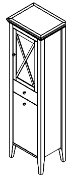
Tall Storage Unit with Laundry Basket 1x Glass Door, 1x Drawer 49x170x39 cm Left CR016 Mahogany CR216 Vintage White Right CR015 Mahogany CR215 Vintage White
